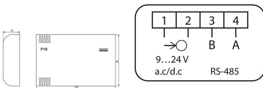
Connection diagram
